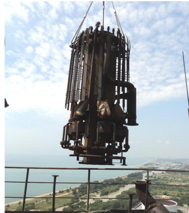
Removal of damaged pilot burner
