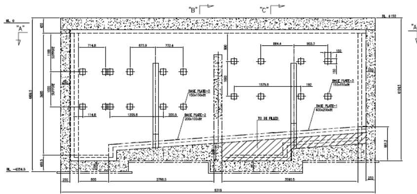
ELEVATION VIEW SCALE 1:25
