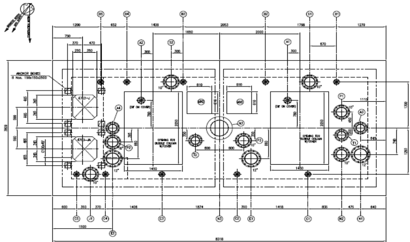
TOP VIEW FOR PIT COVER SCALE 1:25
